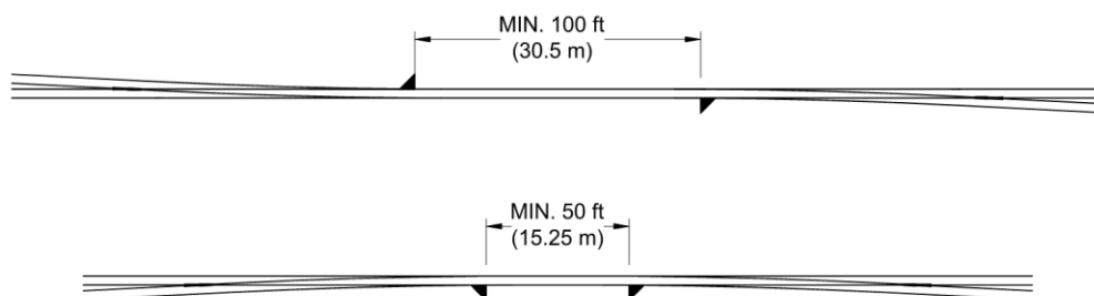
Figure 19-2 Facing Switch Point Separation Requirements
